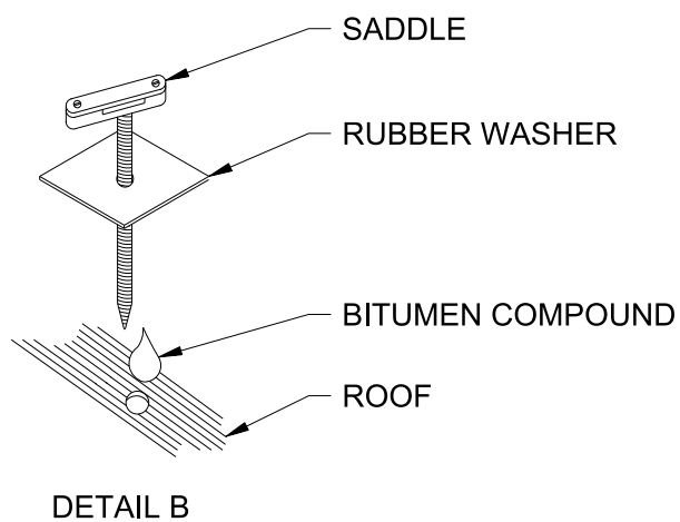
FLATTED ROOF
