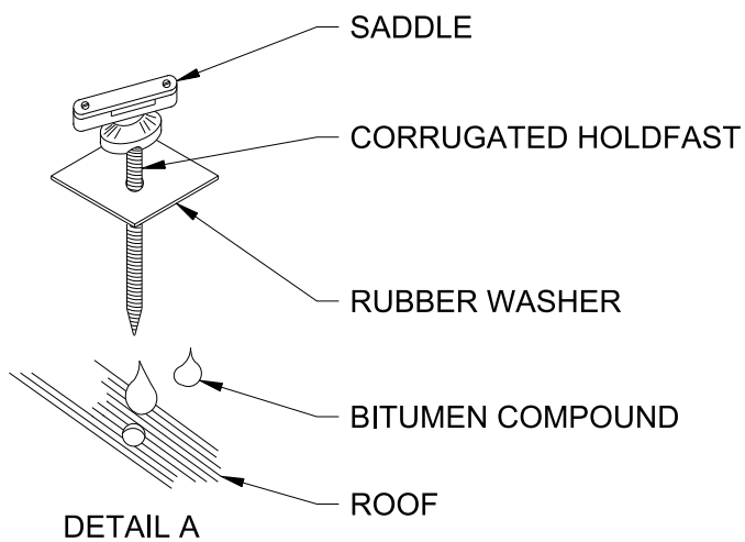
CURVED ROOF
